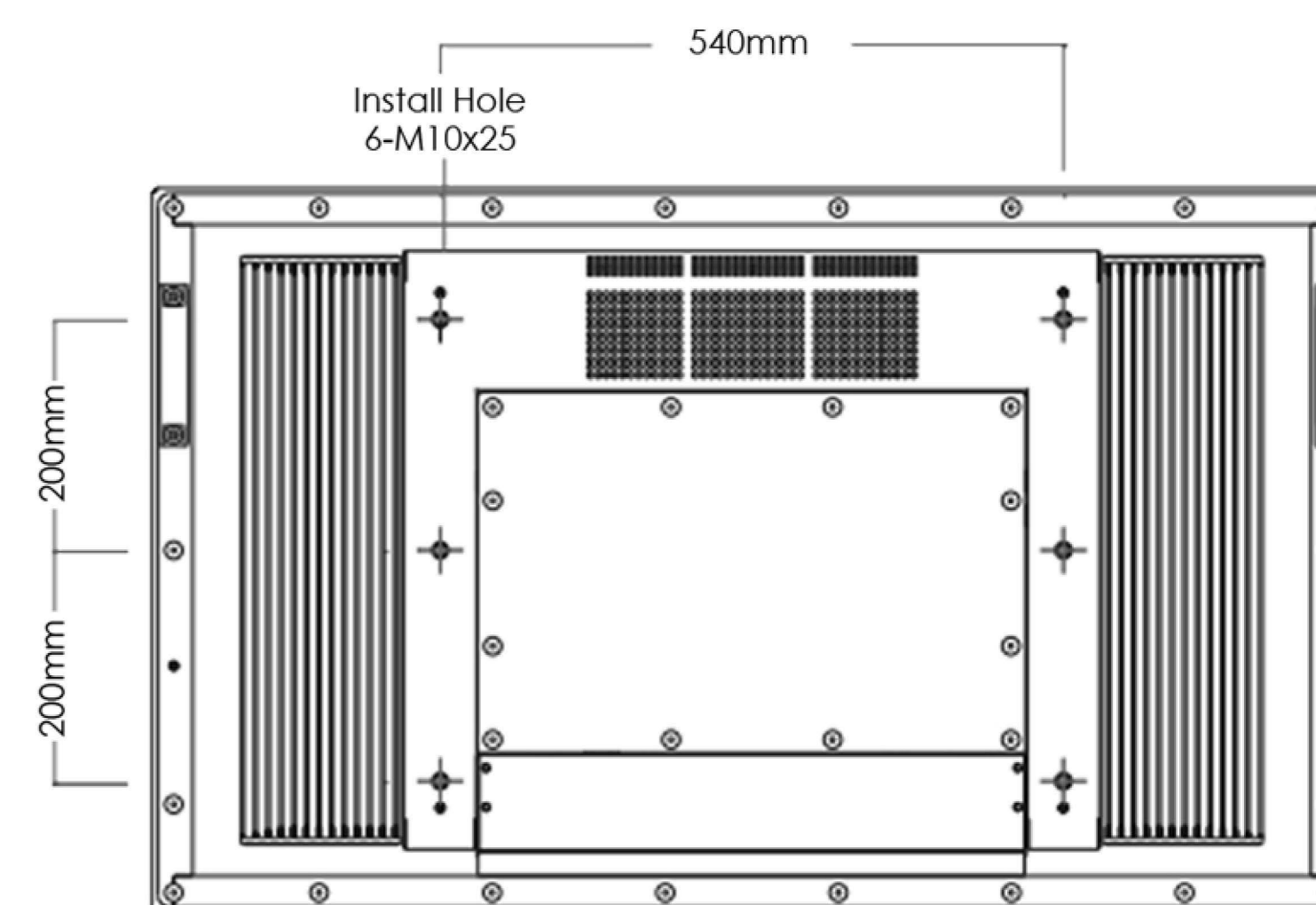
Rear View
