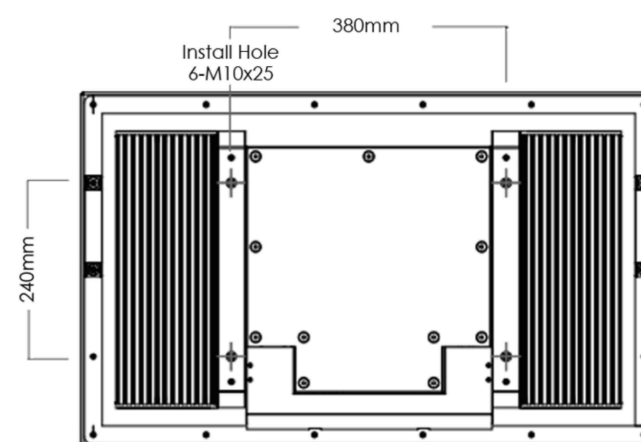
Rear View
